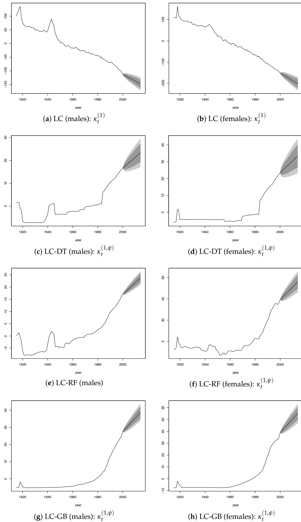
Figure A2. \kappa_t^{(1)} and \kappa_t^{(1,\psi)} : Fitted value (1915–2000) and forecasted values (2000–2014).
