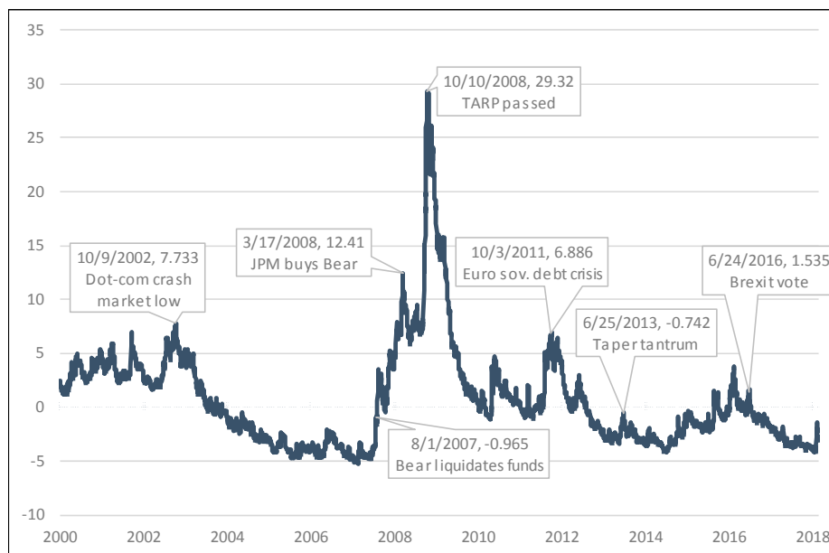
Figure 1. The OFR FSI between January 2000 and December 2018.
