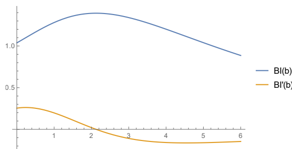
Figure 3. Optimizing dividends with affine drawdown stopping where \mu = 1/2 , q = 1/10 , \sigma = 1 , \xi = 1/3 , b = 20 , d = 1 . The critical point b^* = 2.12445 .
