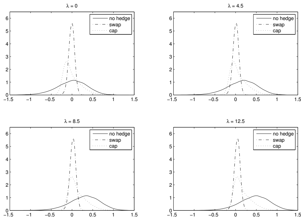
Figure 7. Effect of the longevity risk premium \lambda on the discounted surplus distribution per policy.
