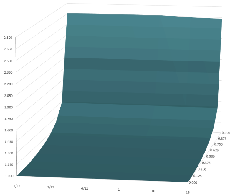
Figure 5. Surface of the ratio Call_t/Call'_t (or Put_t/Put'_t ), displayed on the z axis, for velocities ranging from 0.0\%c to 99\%c (y-axis) and maturities T (x-axis) of 1/12 , 3/12 , 6/12 , 1 , 10 and 15 years. The asset volatility is fixed at \sigma = 15\% . For simplicity, we consider the values at inception t = 0 and r = 0\% and both asset prices at inception and strike equal to one S = K = 1 .
