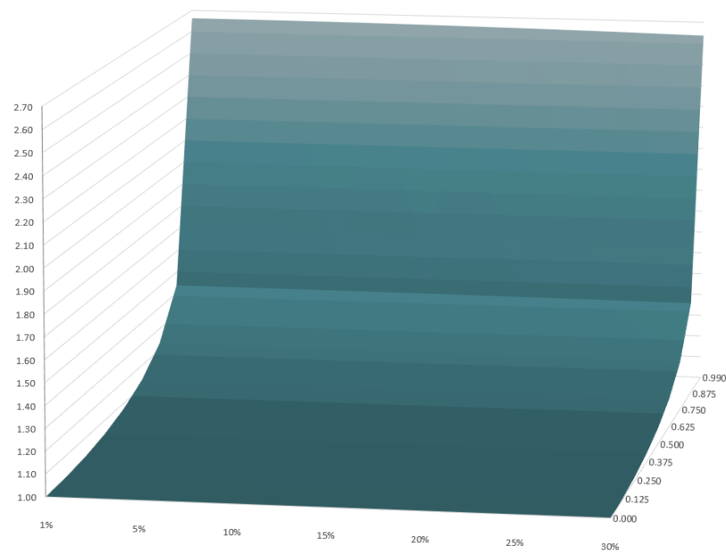
Figure 8. Surface of the ratio Theta/Theta' (for a Call or Put), displayed on the z axis, for velocities ranging from 0.0\%c to 99\%c (y-axis) and the volatilities \sigma (x-axis) of 1%, 5%, 10%, 15%, 20%, 25% and 30%, for maturity T = 1 year. For simplicity, we consider the values at inception t = 0 and r = 0\% and both asset prices at inception and strike equal to one S = K = 1 . Theta' is Theta for a reference frame that is moving and measures less time for velocities >0 . Lemma 7's proof shows that, for a Call or a Put, the Theta/Theta' and Vega/Vega' ratios are equal. Thus, Figure 8 presents both ratios. Vega' is Vega for a reference frame that is moving and measures less time for velocities >0 .
