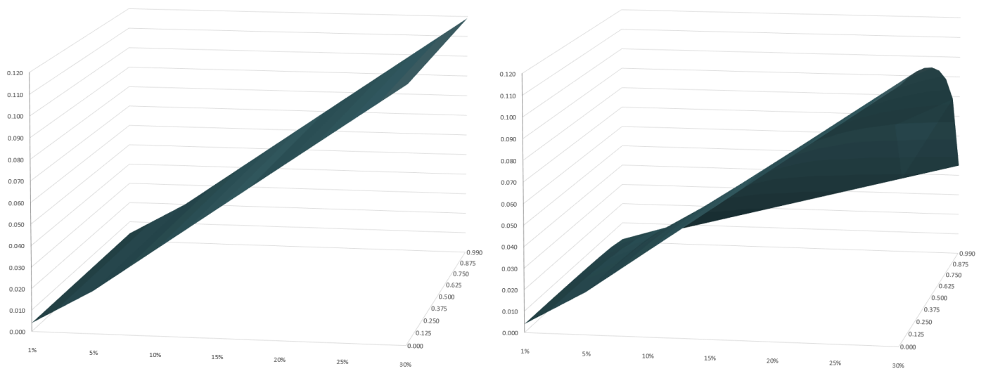
Figure 6. Surfaces of European ATM call (or put) prices (z-axis) in the reference frames L (left figure) and L' (right figure), for velocities ranging from 0.0% to 99% (y-axis) and the volatilities \sigma (x-axis) of 1%, 5%, 10%, 15%, 20%, 25% and 30%, for maturity T = 1 year. For simplicity, we consider values at inception t = 0 , r = 0\% and both asset prices at inception and strike equal to one S = K = 1 .
