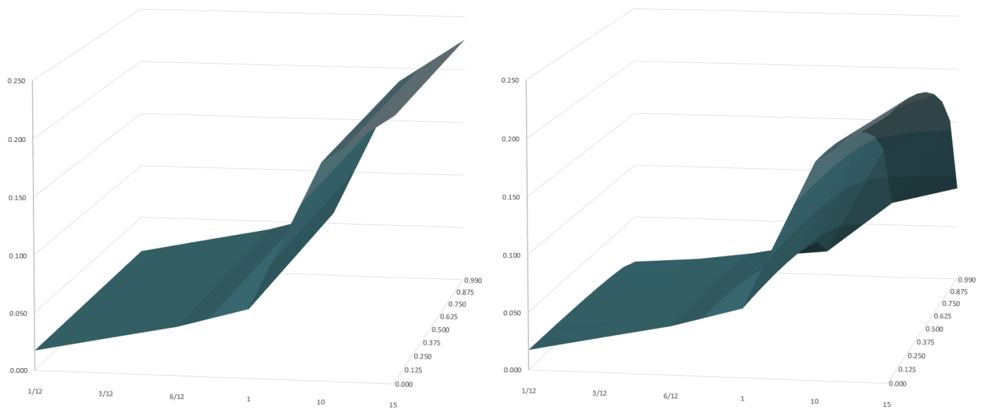
Figure 4. Surfaces of European ATM call (or put) prices (z-axis) in the reference frames L (left figure) and L' (right figure), for velocities ranging from 0.0\%c to 99\%c (y-axis) and maturities T (x-axis) of 1/12 , 3/12 , 6/12 , 1 , 10 and 15 years. The asset volatility is fixed at \sigma = 15\% . For simplicity, we consider the values at inception t = 0 and r = 0\% and both prices at inception and strike equal to one S = K = 1 .
