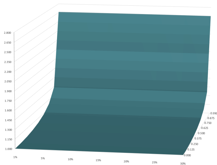
Figure 7. Surface of the ratio Call_t/Call'_t (or Put_t/Put'_t ), displayed on the z axis, for velocities ranging from 0.0% to 99% (y-axis) and volatilities \sigma (x-axis) of 1%, 5%, 10%, 15%, 20%, 25% and 30%, for maturity T = 1 year. For simplicity, we consider the values at inception t = 0 and r = 0\% and both asset prices at inception and strike equal to one S = K = 1 .
