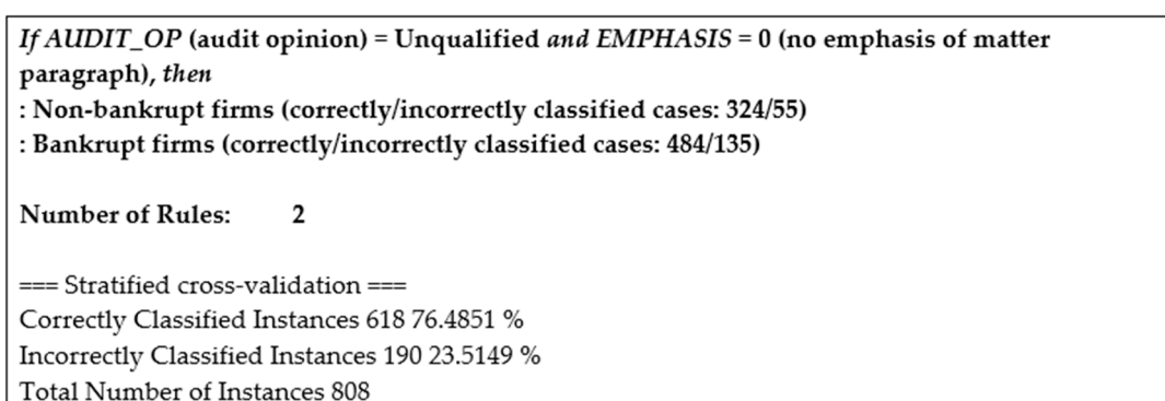
Figure 2. Model 2: The audit opinion and type of paragraphs PART model.
