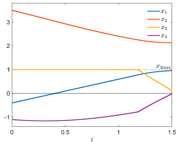
Figure 12. State trajectory.
