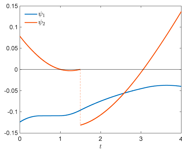
Figure 2. Adjoint trajectory.
