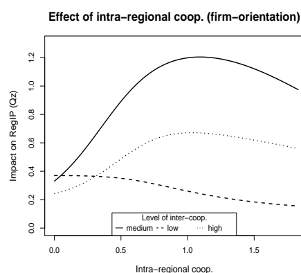
Figure 6: CoopIntra, firm-orient.
