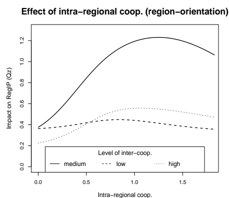
Figure 7: CoopIntra, region-orient.
