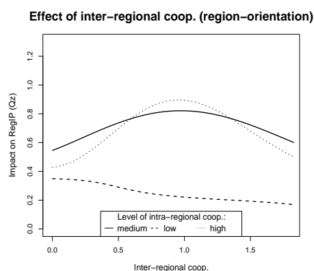
Figure 9: CoopInter, region-orient.
