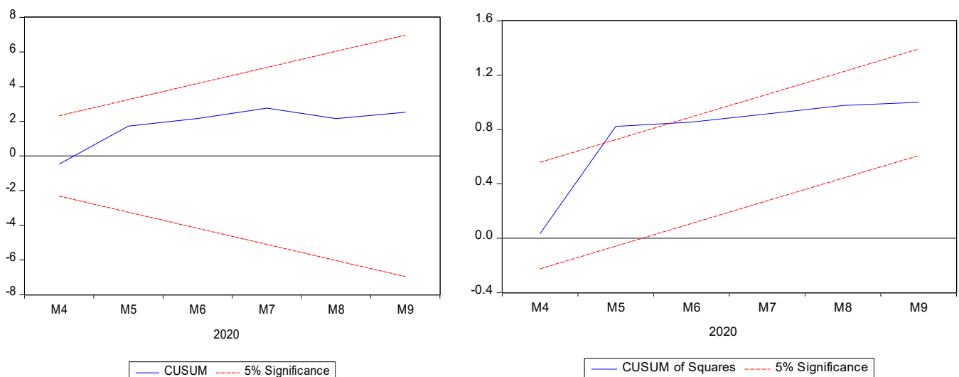
Figure 2. Plot of CUSUM and CUSUMSQ tests for Model 1.
