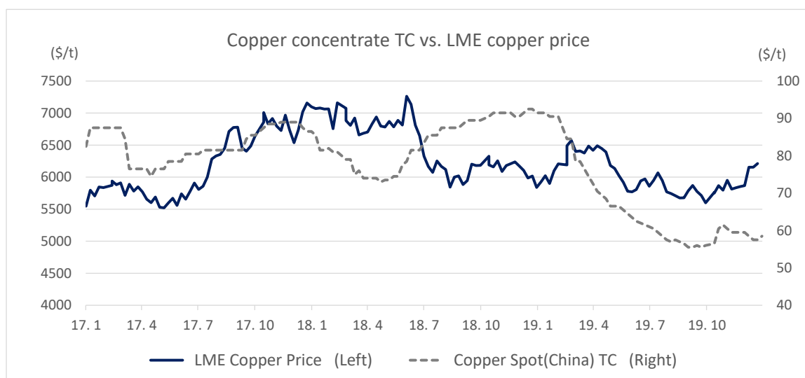
Figure 1. Plot of copper prices and TC.
