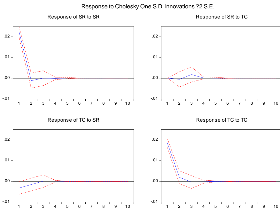
Figure 3. Plot of Impulse Response Results. The solid blue line is the orthogonalized impulse response, while the red dotted line is the 95% confidence interval. The responses of SR to a TC shock show that they were very short lived within second period. The SR is the natural logarithm of weekly returns of copper and TC is the natural logarithm of treatment charge against previous week.
