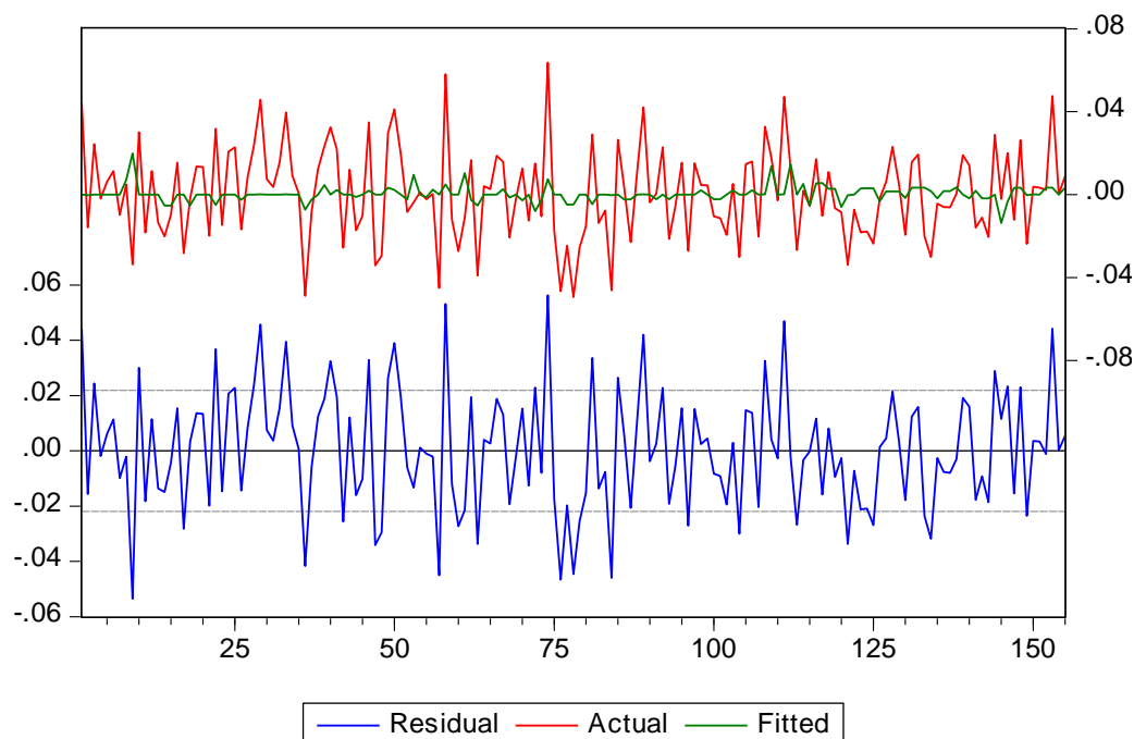
Figure 2. Plot of Residual of Regression Result.
