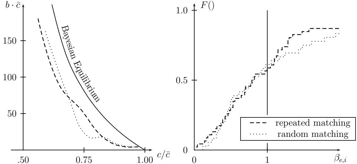
The figure compares bidding with repeated and with random matching. In the left part of the figure we show median bids of the losers (similar to figure 6), in the right graph we show the cumulative distribution of \hat{\beta}_{e,i} (similar to figure 8). In both graphs we show only the case \underline{c} = 2.2 , \bar{c} = 4.4 .
