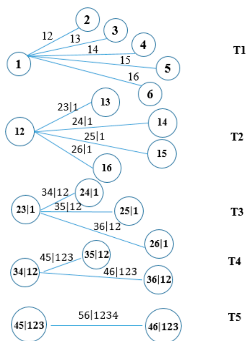
Figure 1. A canonical vine with six variables, five trees and 15 edges.
