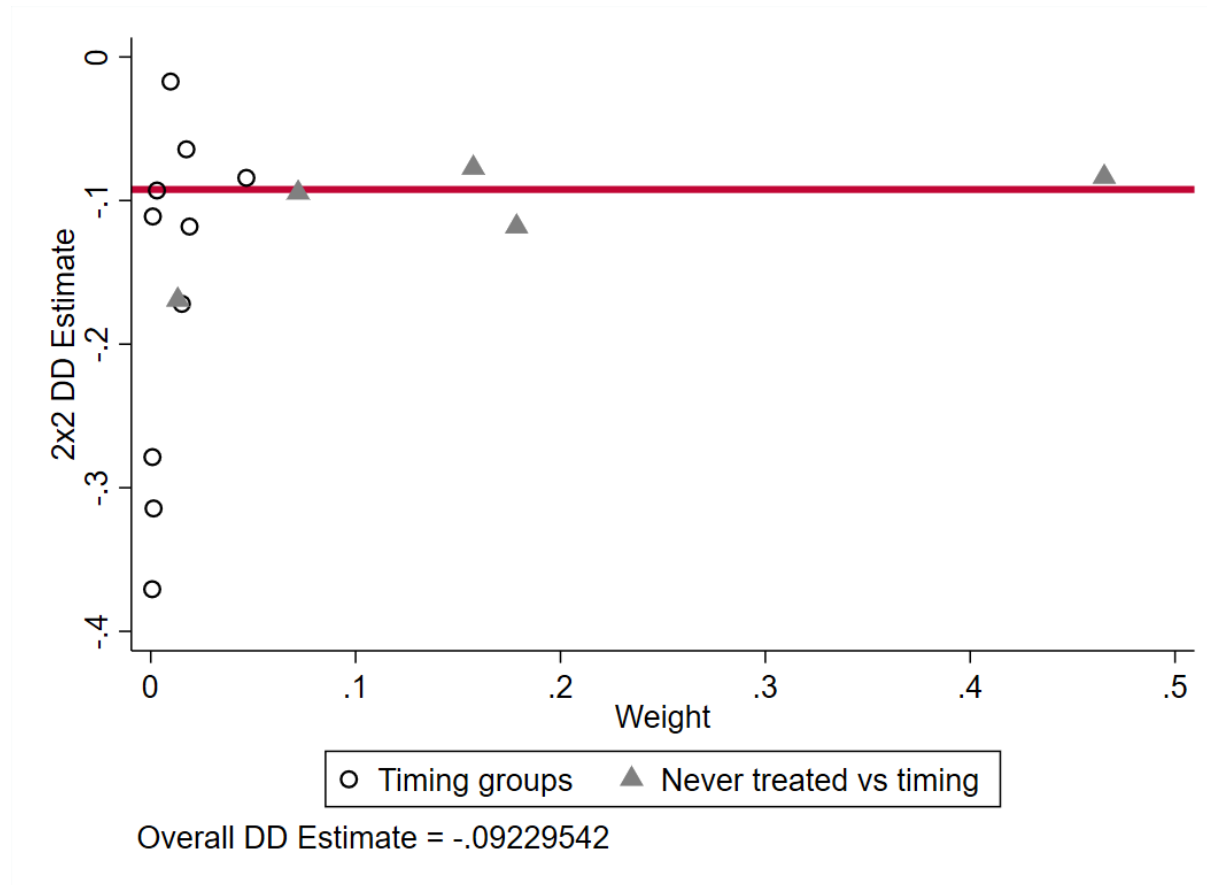
Figure 3: Goodman-Bacon Decomposition
