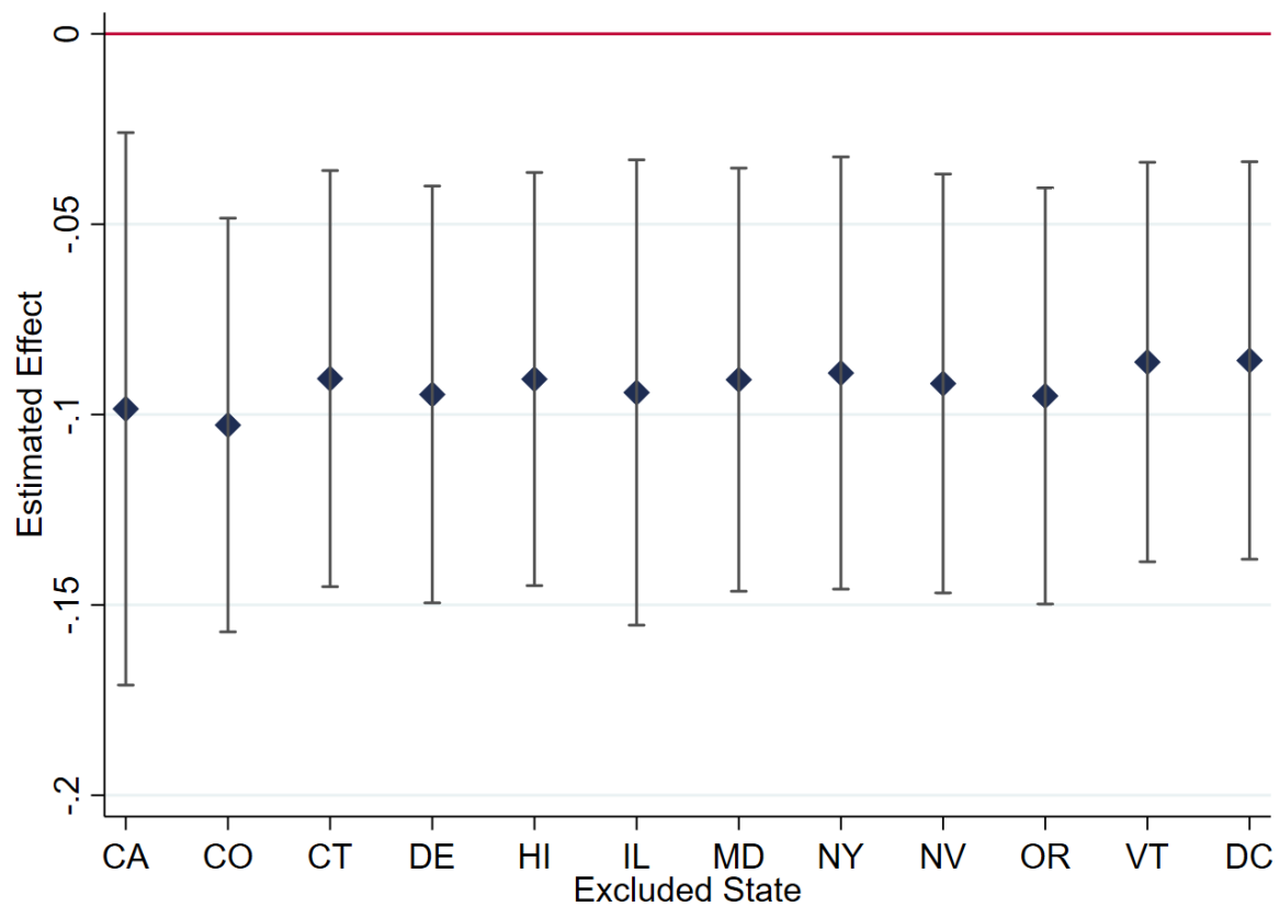
Figure 2: Leave-one-out Analysis
