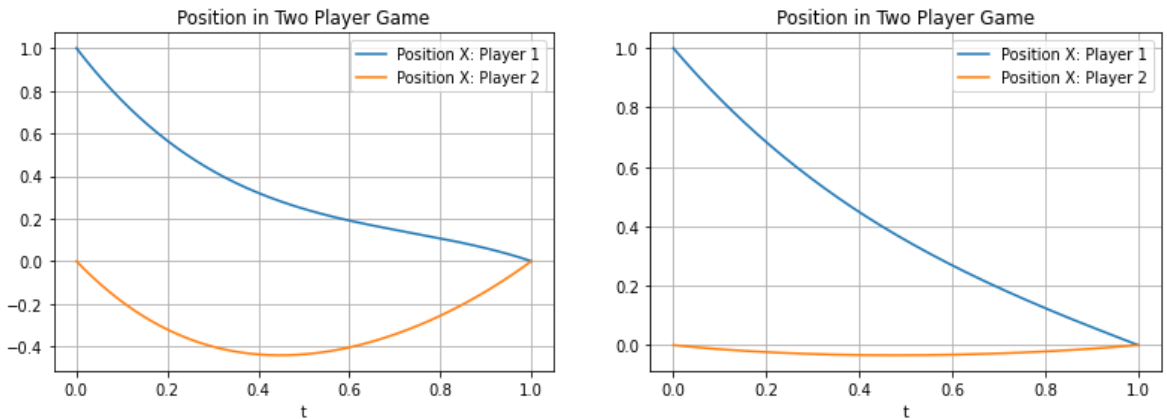
Figure 3: Portfolio process in the two player game under different parameters \gamma , \gamma = 1 (left) and \gamma = 0.1 (right). Other parameters are chosen as \eta_1 = \eta_2 = 0.1 , \rho_1 = \rho_2 = 0.2 , \lambda_1 = \lambda_2 = 0.3 , \alpha_1 = \alpha_2 = 1 , \beta_1 = \beta_2 = 1.1 , x_1 = 1, x_2 = 0 , and T = 1 .
