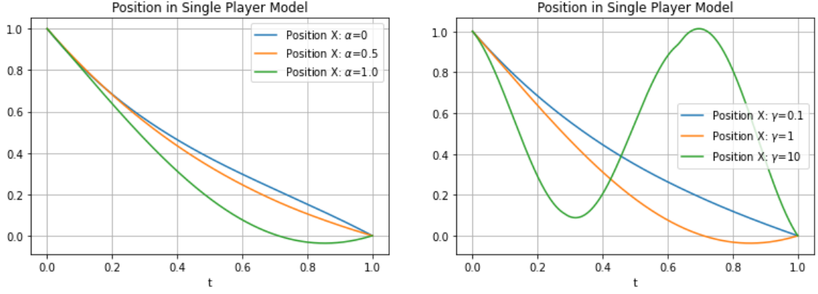
Figure 2: Dependence of optimal portfolio process on the market impact parameters \alpha and \gamma , \gamma = 1 (left) and \alpha = 1 (right). Parameters are chosen as \eta = 0.1 , \rho = 0.2 , \lambda = 0.3 , \beta = 1.1 , x = 1 and T = 1 .
