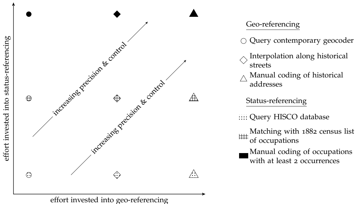
Figure 4: Effort-precision trade-offs
