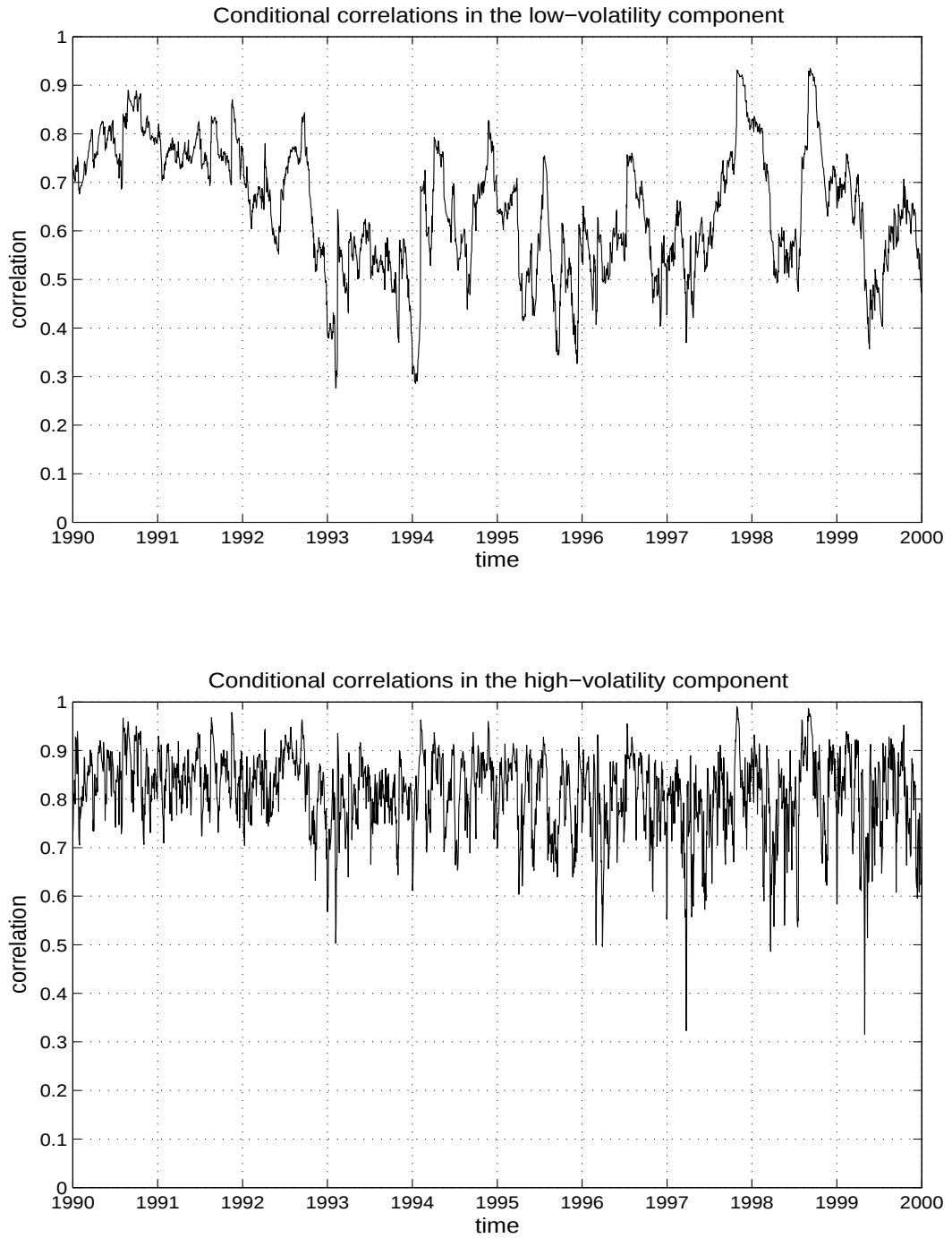
Figure 1: Shown are the implied component-specific correlations of the MNM(2)–GARCH(1,1) model, fitted to the NASDAQ/DJIA returns. The upper panel shows the conditional correlations in the low-volatility component, those in the high-volatility component are depicted in the lower panel.
