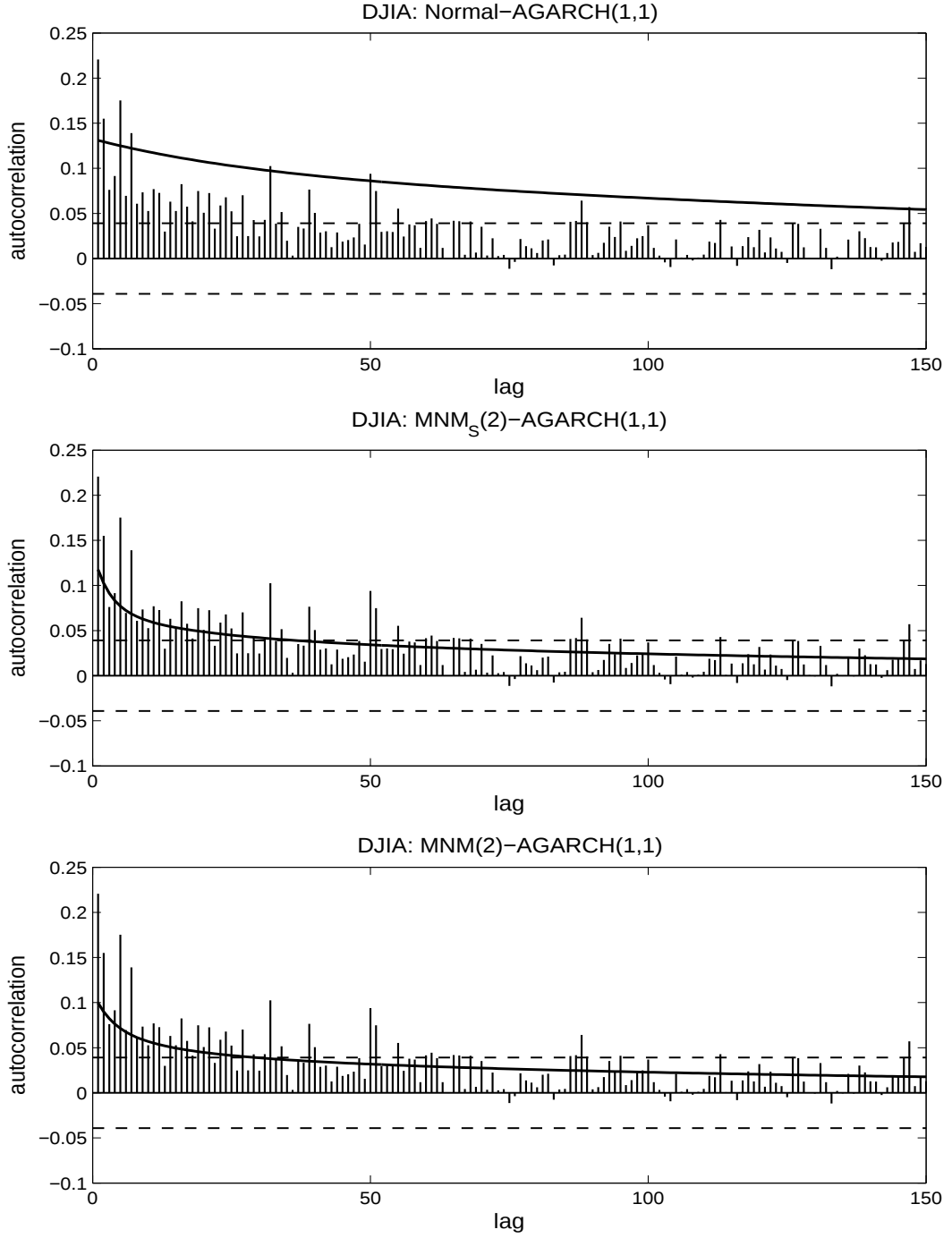
Figure 5: Shown are the empirical autocorrelations (vertical bars) of the squared (filtered) DJIA returns, as well as their theoretical counterparts (solid lines), as implied by the fitted Normal-AGARCH(1,1) (top panel), MNM_S(2) -AGARCH(1,1) (middle panel), and MNM(2) -AGARCH(1,1) (bottom panel) models. The usual 95% asymptotic confidence intervals (dashed lines) associated with a white noise process with finite second moment are also included.
