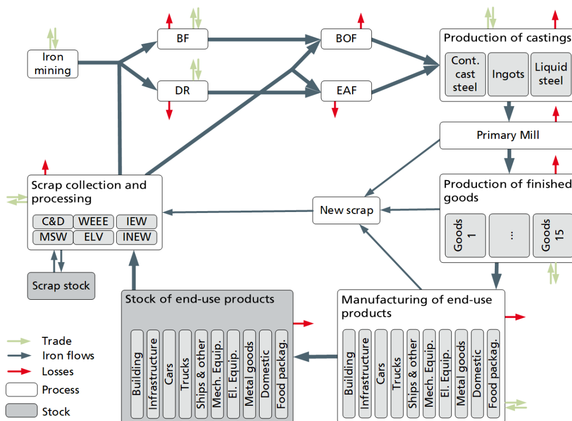
Figure 1: Scheme of the European steel cycle.
