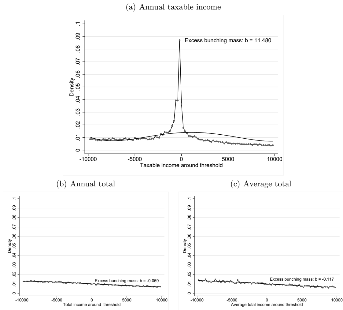
Figure 4.1: Bunching around the higher rate threshold
