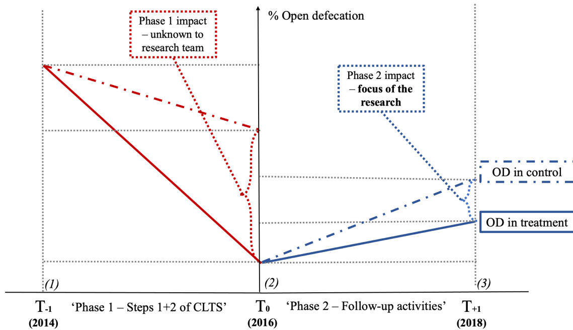
Figure 1: Research design
