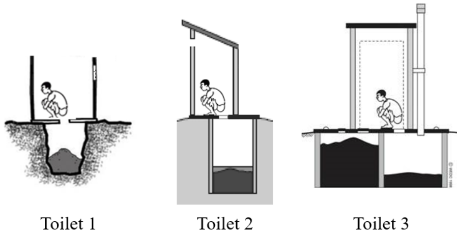
Figure 1 Toilet types
