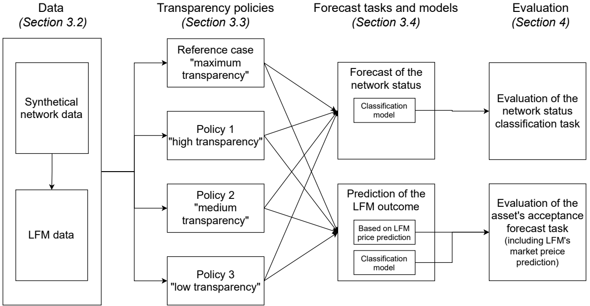
Figure 1: Method overview
