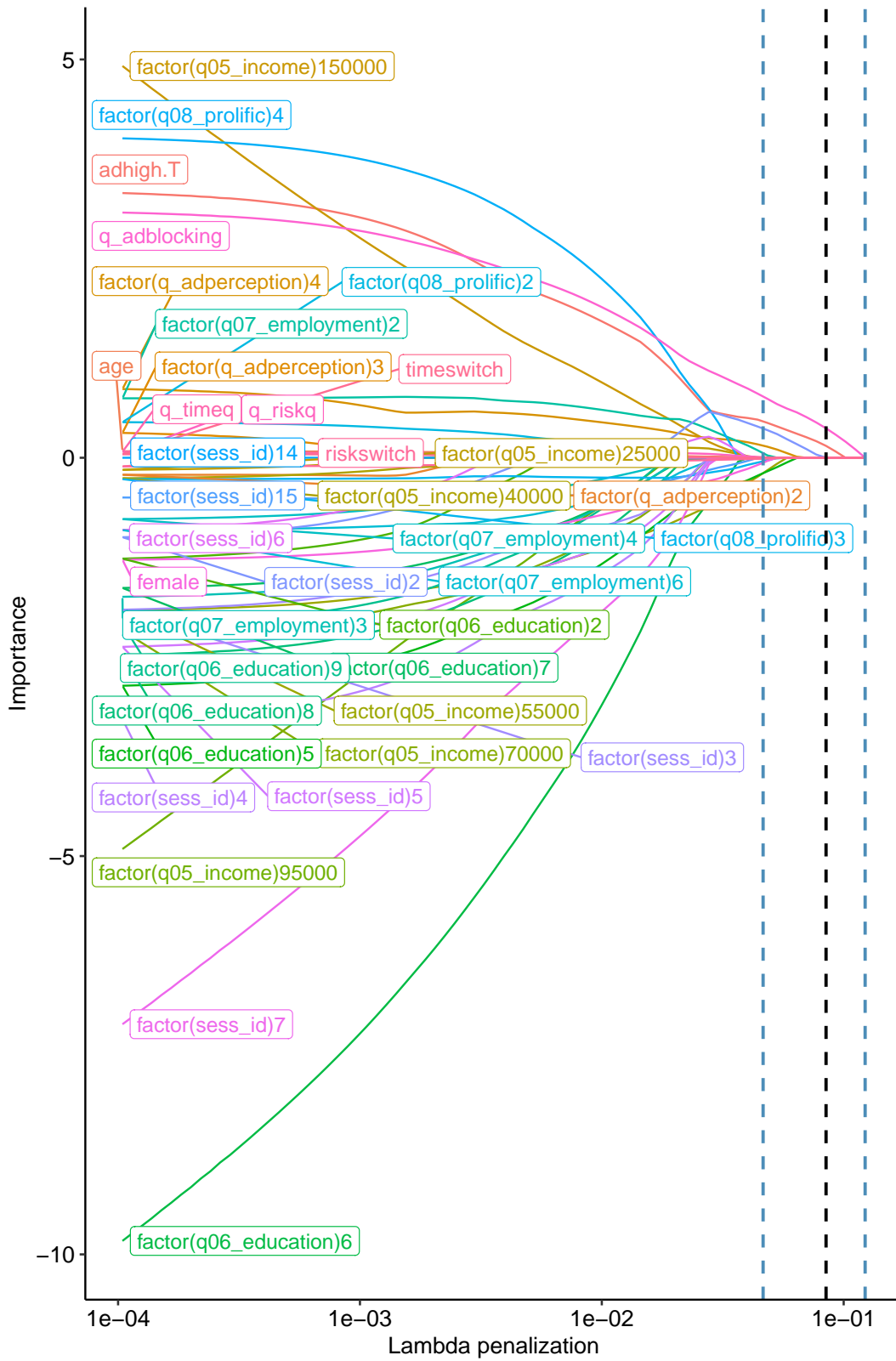
Figure 15: Lasso lambda penalization convergence
