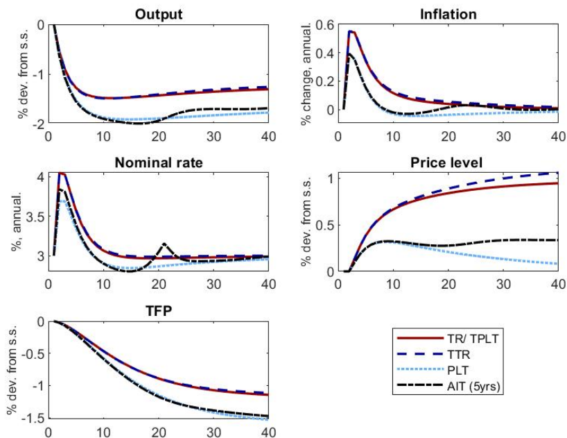
Figure 9: Impulse responses to inflationary supply shock.
