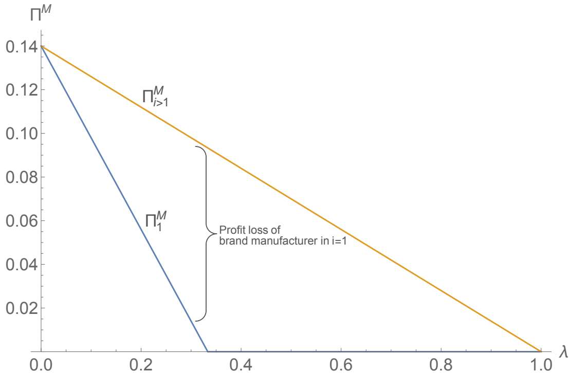
Figure 2: Manufacturer profits as a function of \lambda . The parameters used are q_H = 1 , c_H = 0.6 , q_L = 0.65 , c_L = 0.53 , I = 4 .
