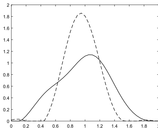
FIGURE 4. Cross-sectional distribution of market betas at open and close of trading. The plot displays \hat{f}_{T,\kappa}^\beta(x) using the first two hours of trading (solid line) and the last 2 hours of trading (dashed line), both computed over the entire sample. The tuning parameter u_n in the Fourier inversion is set to \inf\{0 < u : |\mathcal{L}_{T,\kappa}^\beta(u)| < 0.0005\} .
