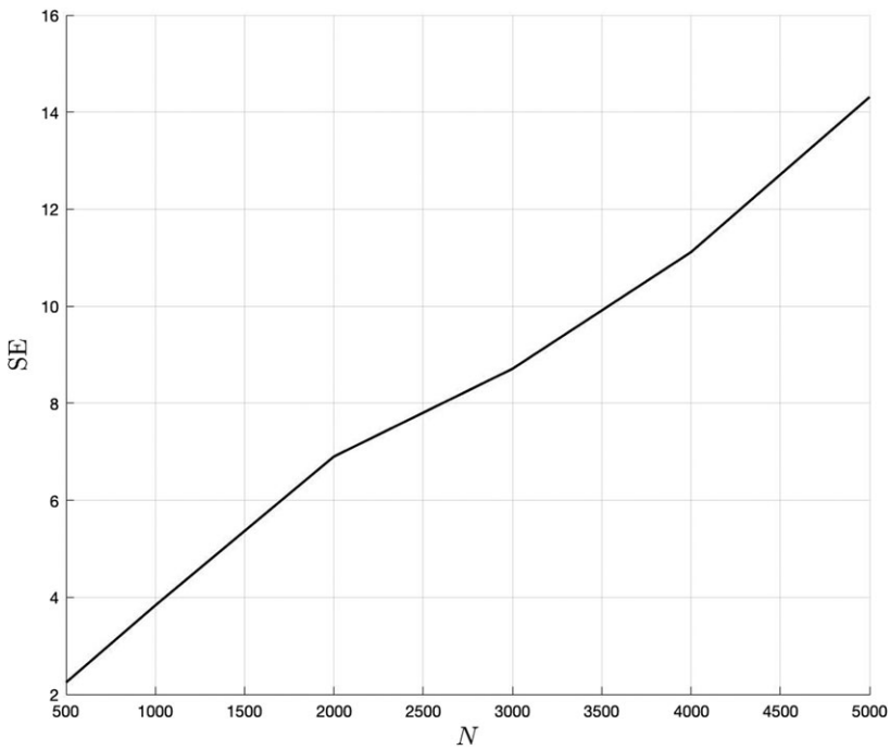
FIGURE 10. Standard errors versus sample length (Computations based on J = 1000 independent runs for each N ). Random walk: \tilde{x}_{t+1} = x_t + \tilde{\varepsilon}_{t+1} , \{\tilde{\varepsilon}_{t+1}\} \sim N(0, \sigma_\varepsilon^2) , \sigma_\varepsilon = 0.00712 .
