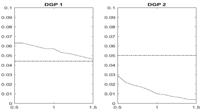
Note: Rejection probabilities for BCD assignment rule with n = 200, \pi = 0.5 , and \tau = 0.5 . The X-axis is C_f . The solid lines are the rejection probabilities for “s/adj”. The densities of Y_j is computed using the tuning parameters h_j = 1.06C_f\hat{\sigma}_jn_j^{-1/5} , for j = 0, 1 . The dotted dash lines are the rejection probability for “s/CA”.
