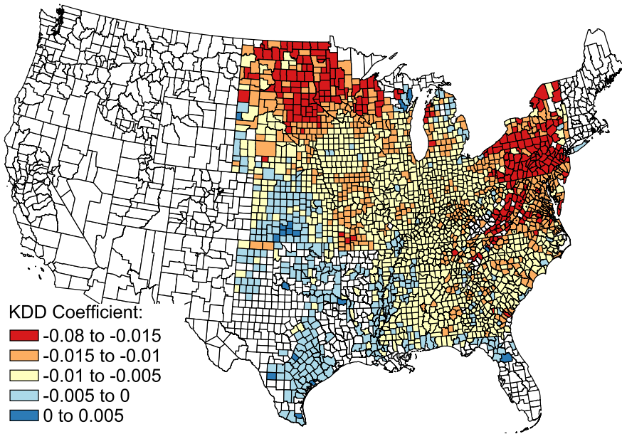
FIGURE 3. Distribution of KDD slope coefficients across counties for U.S. corn. Note: This graph maps for each country of the United States in the estimation sample the average value of \hat{\beta}_{2it} from the MO-OLS model (see Table 2).
