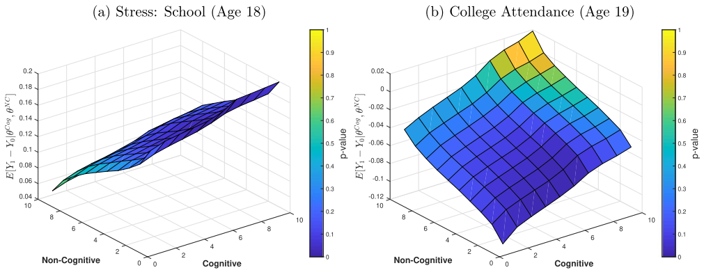
FIGURE 4. ATE of being bullied at age 15 on educational outcomes at age 18 and older. Note: Panels display ATE(\theta^{NC}, \theta^C) = \mathbb{E}[Y_1 - Y_0 | \theta^{NC}, \theta^C] in the z -axis resulting from 40,000 simulations based on the findings of the empirical model. The x -axis and y -axis contain the deciles of noncognitive and cognitive skills, respectively. “Stress: school” is a variable that aggregates stress symptoms triggered by situations related with school. “College Attendance” takes the value of 1 if the respondent attends college by age 19.
