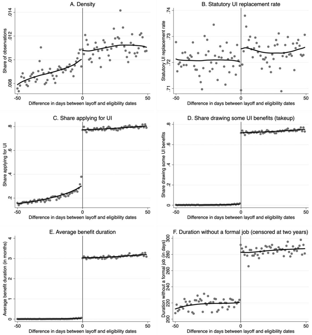
FIGURE 2. Graphical evidence for our empirical application. Notes: The figure displays the mean of different variables on each side of the cutoff by day between the layoff and eligibility dates, and local linear regressions on each side of the cutoff using an edge kernel and a bandwidth of 30 days. The figure is based on a sample of 169,575 displaced formal workers whose layoff date fell within 50 days of the eligibility date.
