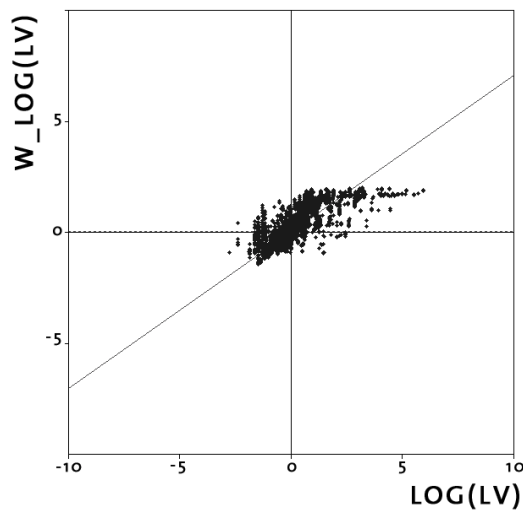
Fig. 2a Spatial Dependence with 3000 meter Specification
