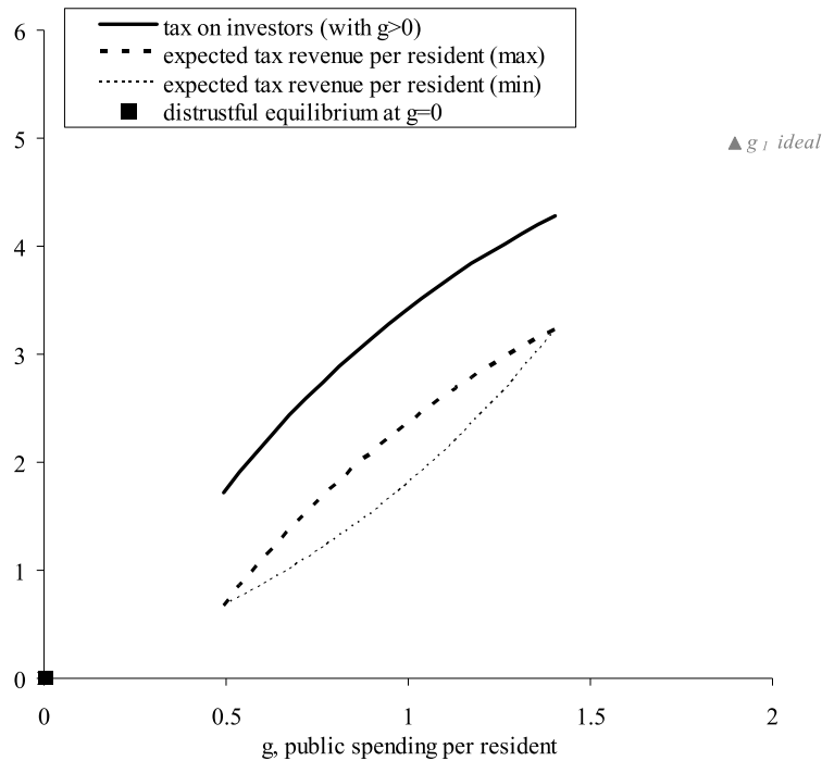
FIGURE 1. Possible equilibrium levels of public spending g , with the corresponding tax \tau on investors, and the potential expected tax revenue \tau\varphi per resident, in centralized autocracy, for an example with \pi(g) = 1 - e^{-g} , S = 7 , k = 1 , \beta = 0.95 , \delta = 0 ; compared to the ideal g_1 in local democracy.
