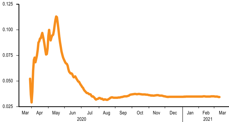
Figure 3: COVID-19 cumulative case fatal rate, 27/3/2020-10/3/2021
