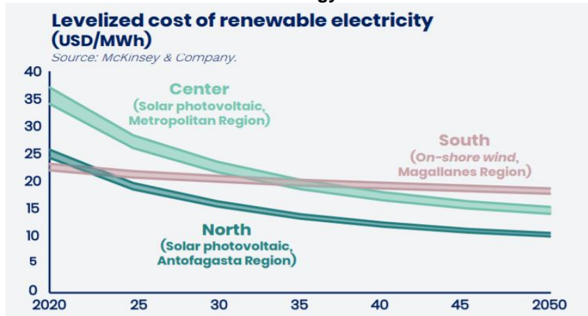
Figure 19: Chile Levelized cost of renewable energy
