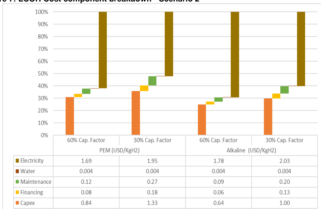
Figure 7: LCOH Cost component breakdown - Scenario 2
