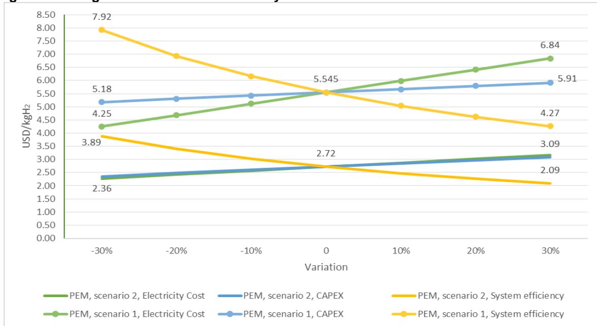
Figure 8: Changes in LCOHs - PEM electrolyzer
