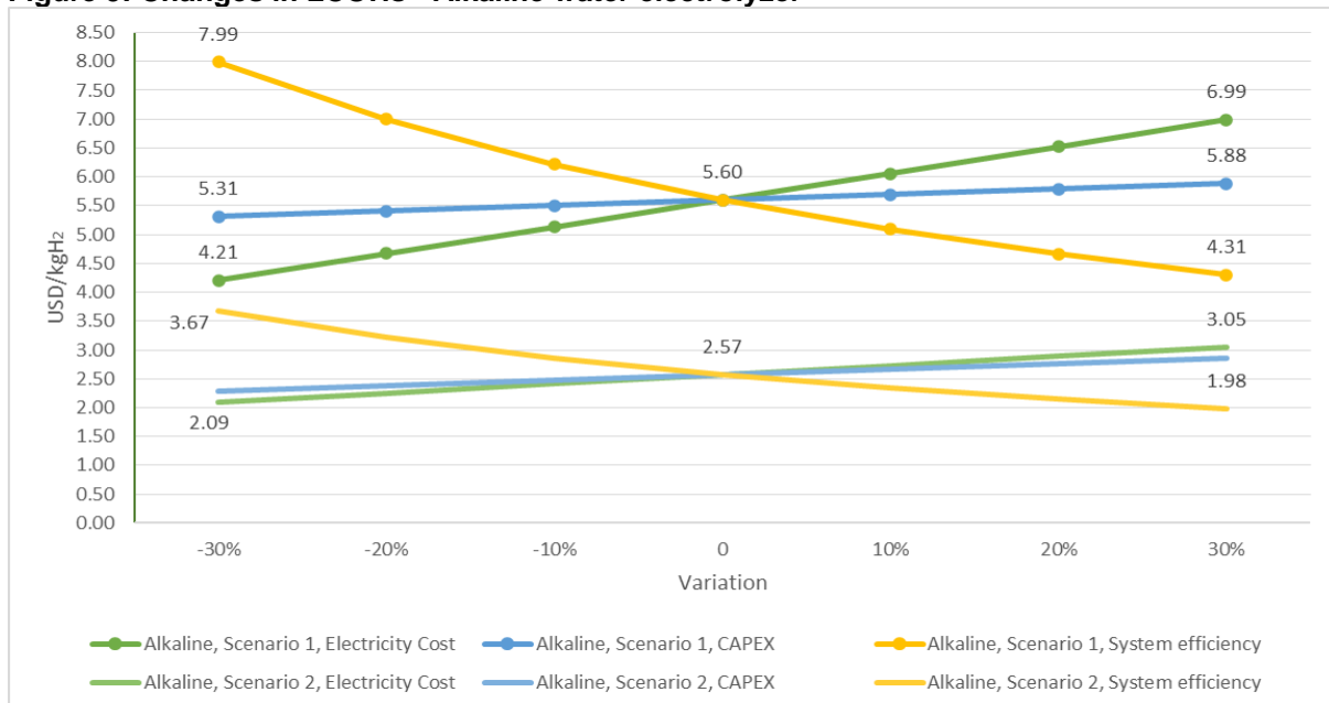
Figure 9: Changes in LCOHs - Alkaline water electrolyzer
