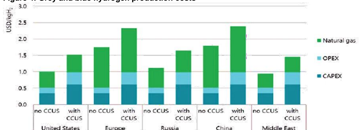
Figure 4: Grey and blue hydrogen production costs
