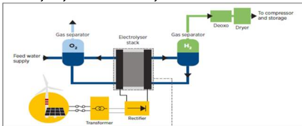
Figure 5: Electrolyzer system level as defined by IRENA
