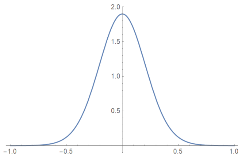
Figure 1. A density function.
