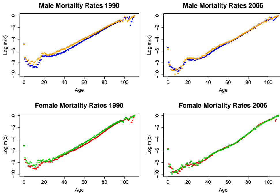
Figure 1: Logarithmic death rates versus age group(0-110) for males (upper figures) and females (bottom figures) in 1990 and 2006 for former West Germany (circles) and East Germany (triangles).
