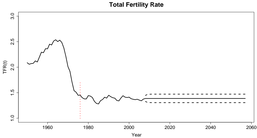
Figure 8: Total Fertility Rates from 1950 – 2007 and the forecast to 2057 concerning data from 1976 only (dotted red line) with the 95%-confidence interval.
