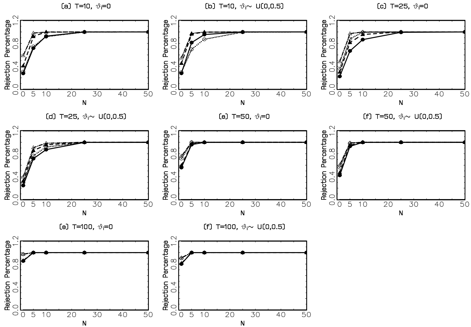
Figure 6: Empirical size-adjusted power results of the tests for DGP C and true cointegrating rank of one when the hypothesized rank is zero. \bullet — panel SL-asymp, \blacktriangle - - - panel SL-VAR(1), \circ ..... LLL-asymp, \Delta - · - · - LLL-VAR(1).
