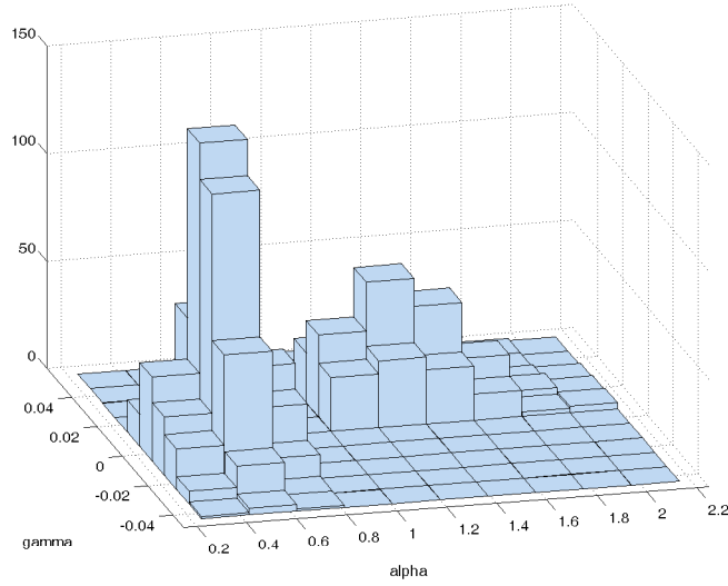
Figure 1: Prior distribution
