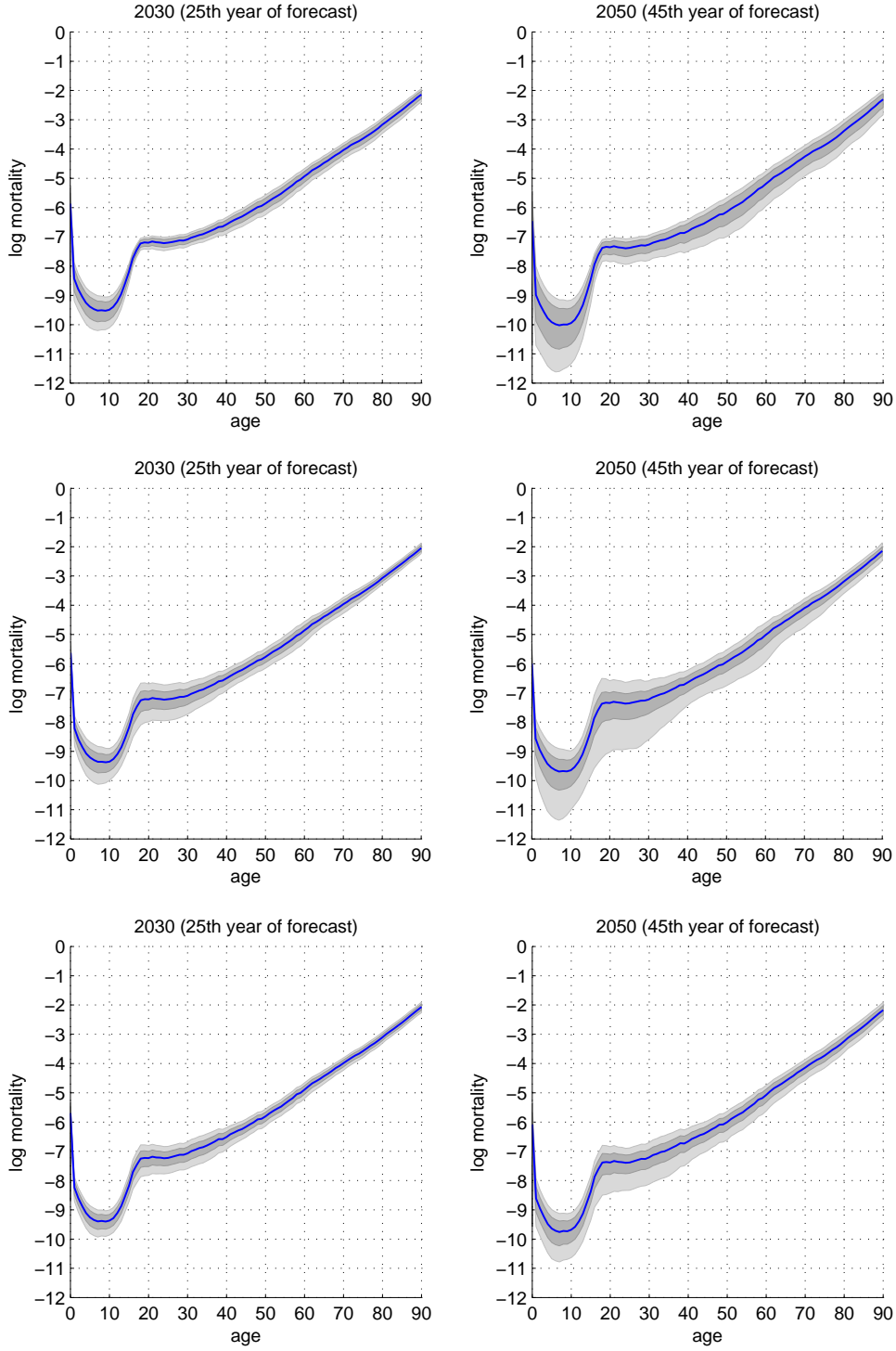
Figure 8: Panel with forecasts of age-specific mortality m_{x,t} 25 and 45 years ahead for different model specifications. The first row shows the specification for K = 1 , N = 0 , the second row for K = 1 , N = 2 , and the third row for K = 2 , N = 2 . The entire gray shaded area around the blue median represents 90% of the posterior probability mass and the dark gray shaded area represents 68% of the posterior probability mass regarding both parameter and random term uncertainty.
