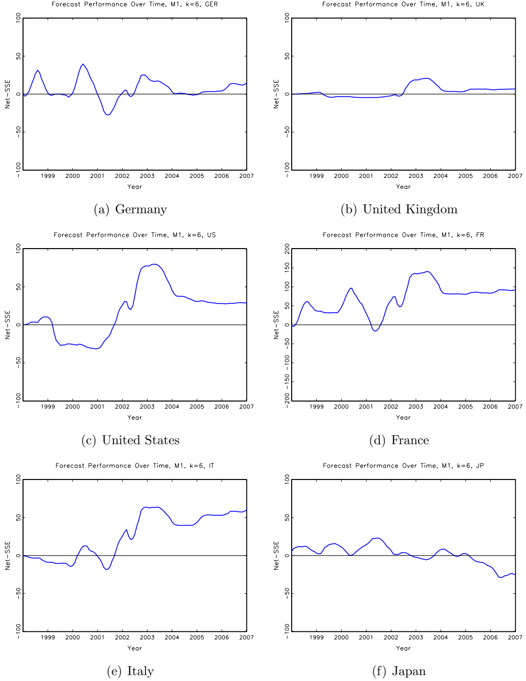
Figure 2: Net-SSE Plots
