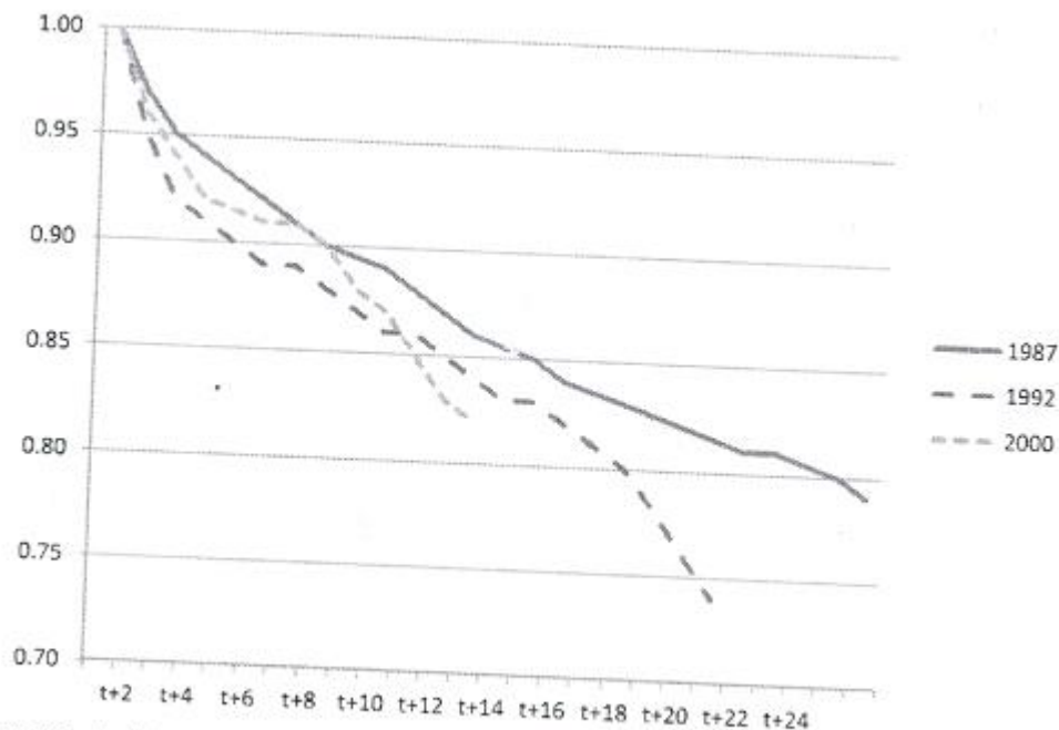
Fig. 2 Survival depends on the timing of labour market entry
