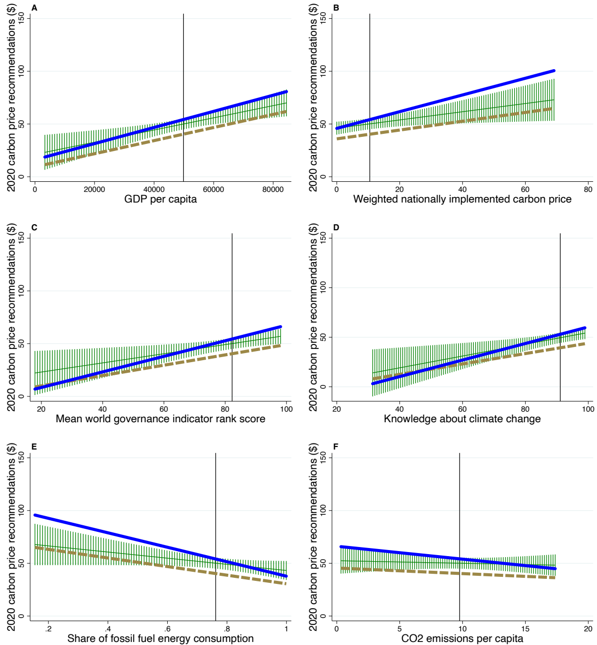
Figure A.5.5: Unilateral and global carbon price recommendations and country characteristics
