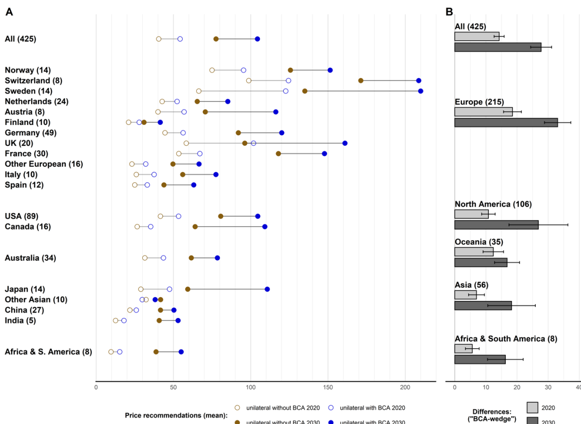
Figure 4: Unilateral carbon pricing and the Border Carbon Adjustment (BCA) wedge
