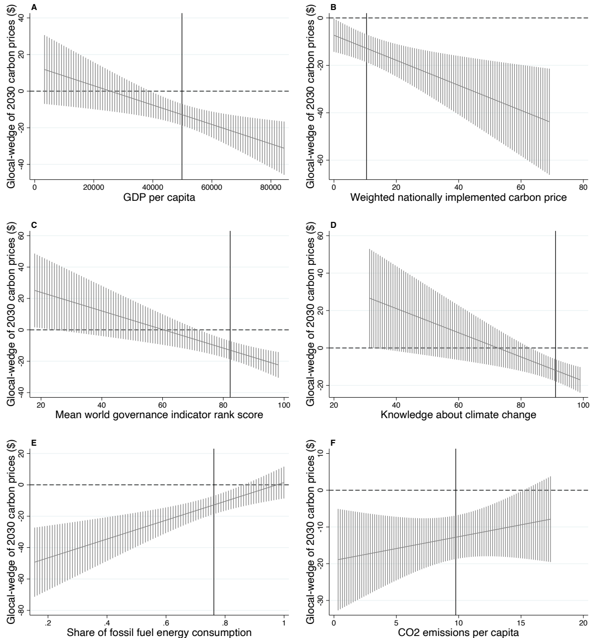
Figure 11: Glocal-wedge of carbon price recommendations and country characteristics
