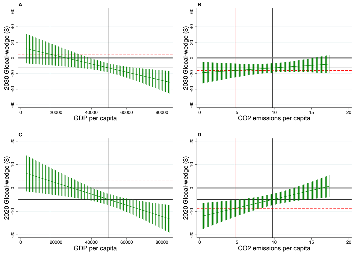
Figure A.6.4: Re-weighting the Glocal-wedge for global GDP and CO2 emissions per capita
