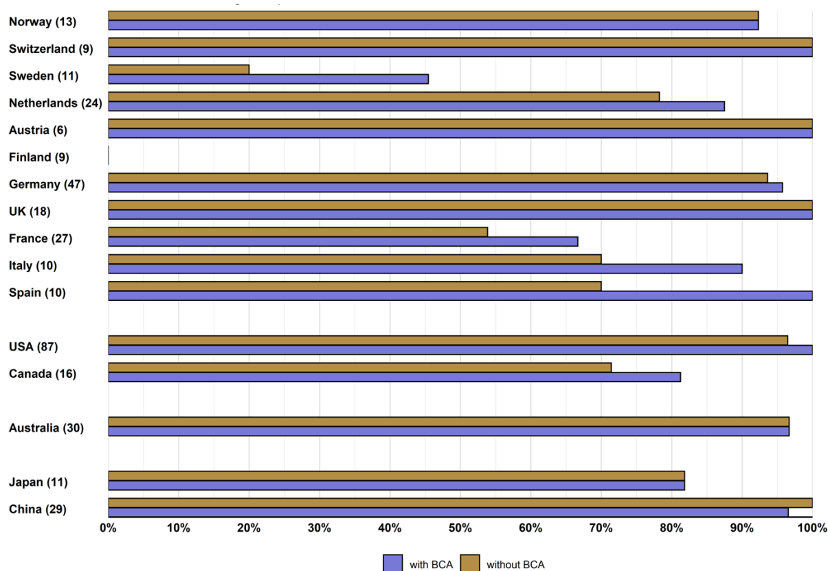
Figure A.4.4: Acceptable ranges of 2020 unilateral carbon prices vs. weighted implemented prices at a country-level
