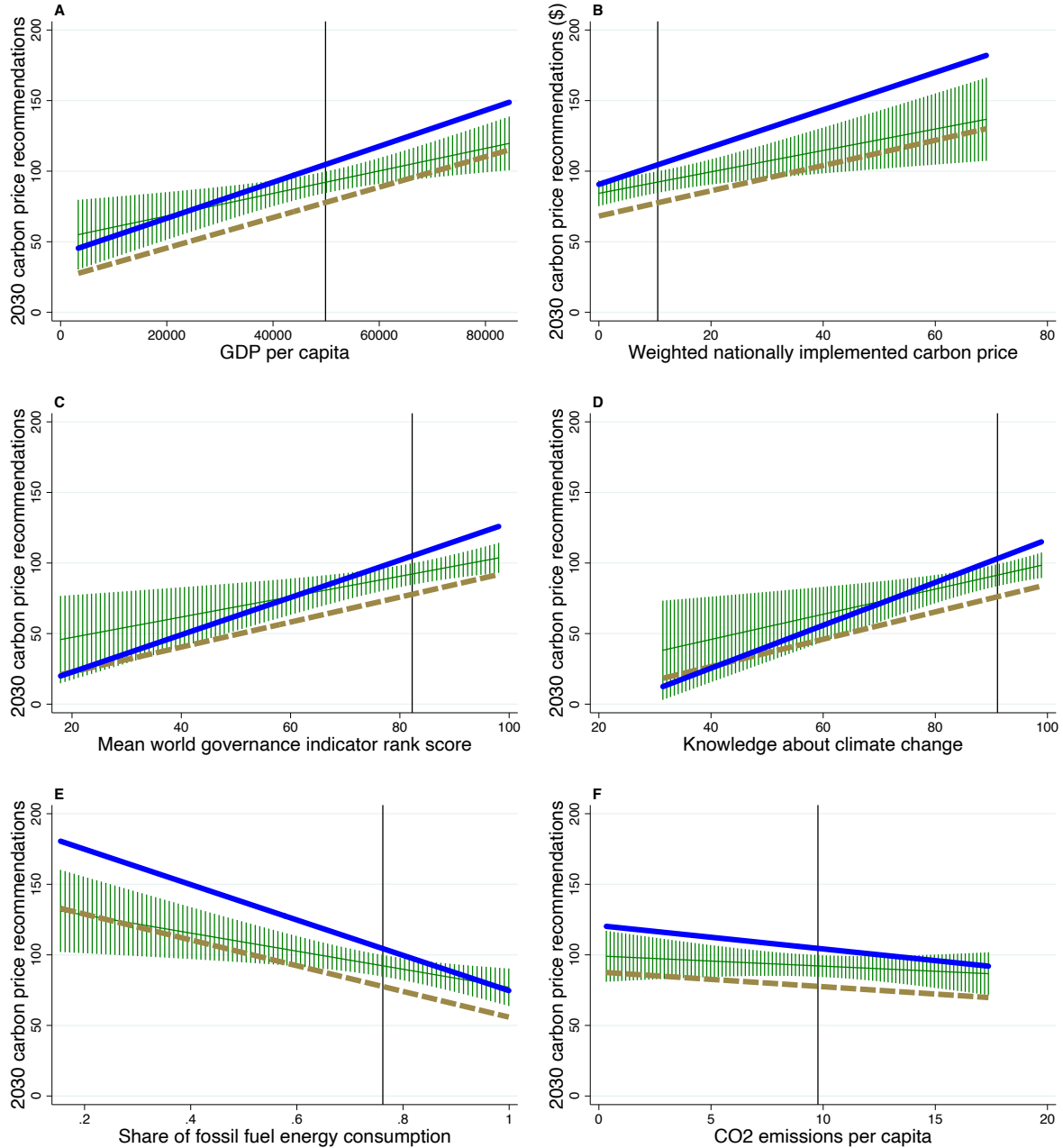
Figure 10: Unilateral and global carbon price recommendations and country characteristics
