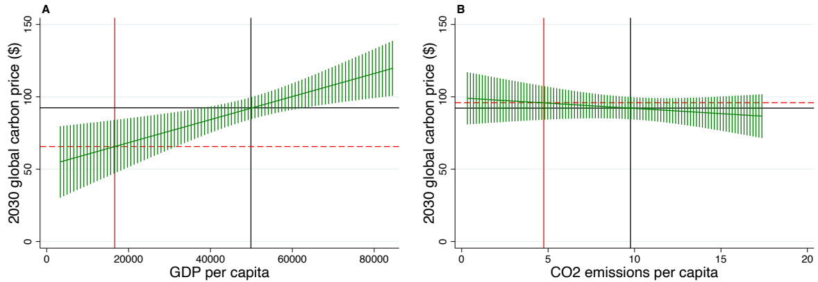
Figure 13: Re-weighting global carbon prices for non-representation bias
