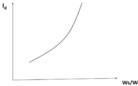
Figure 4: Relationship between unskilled labor demand and skill-unskilled relative wage
