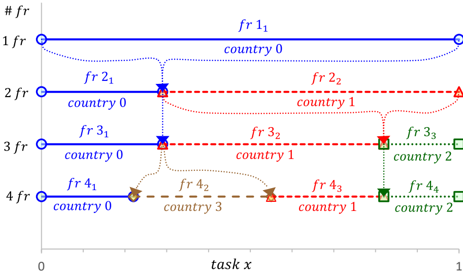
Figure 7 Step-wise fragmentation
