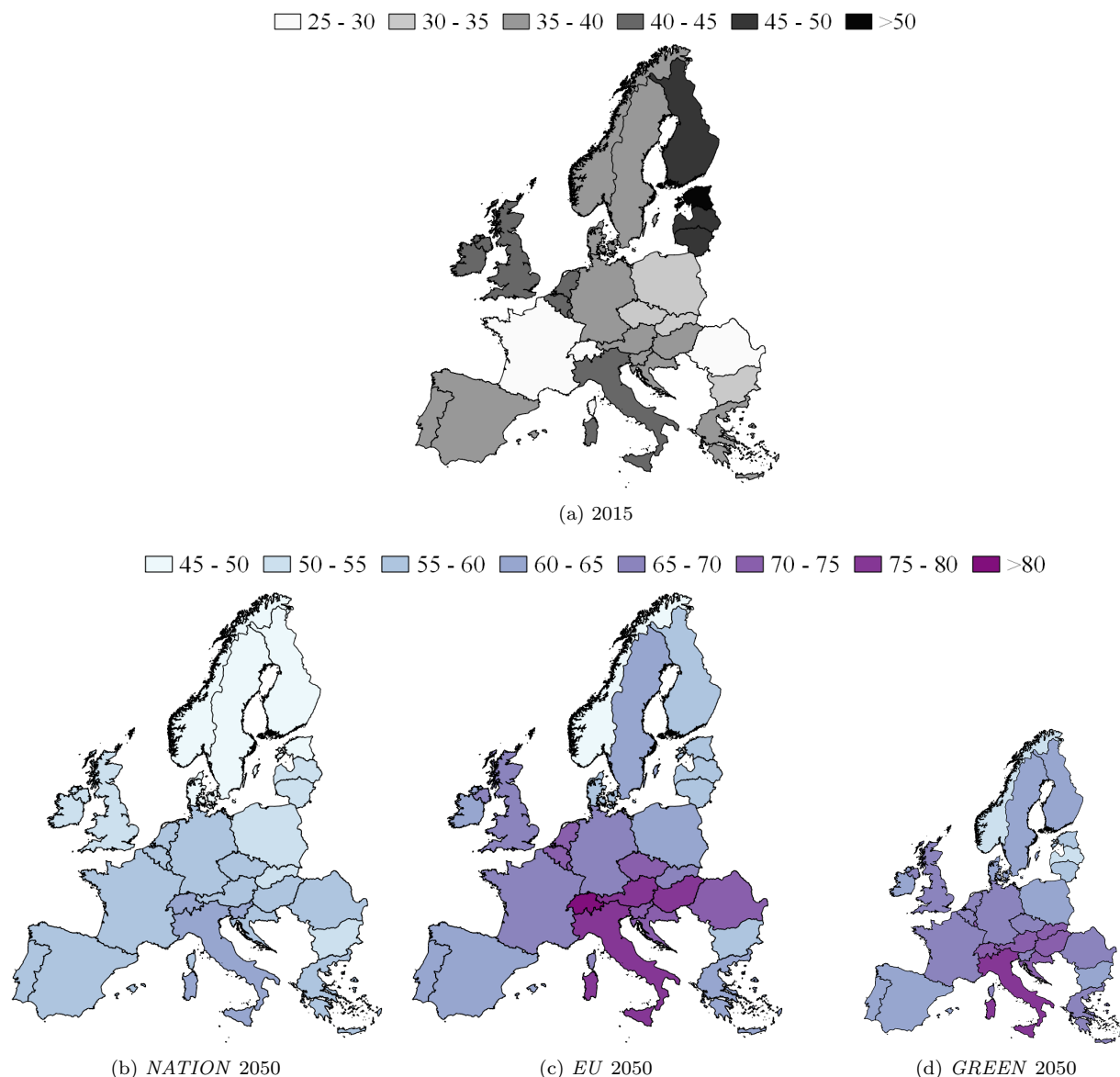
Figure 5: Electricity price (€/MWh) for European countries in 2015 and 2050 across the three narratives NATION , EU , and GREEN
