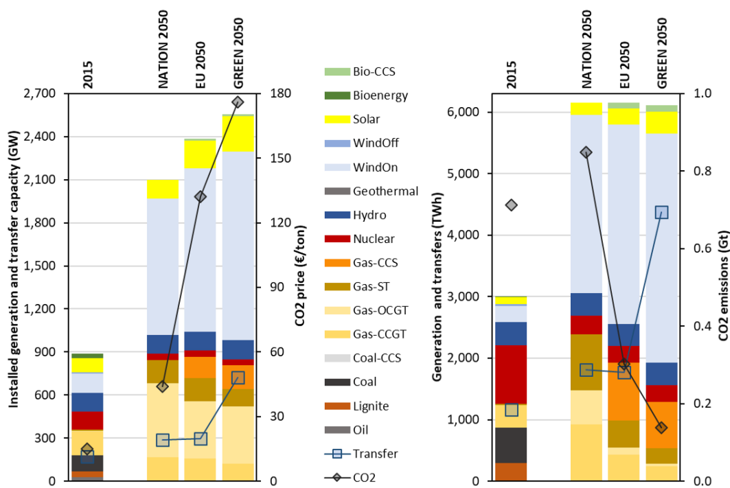
Figure 3: Technology mix, transfer volume, and resulting decarbonization by narrative
