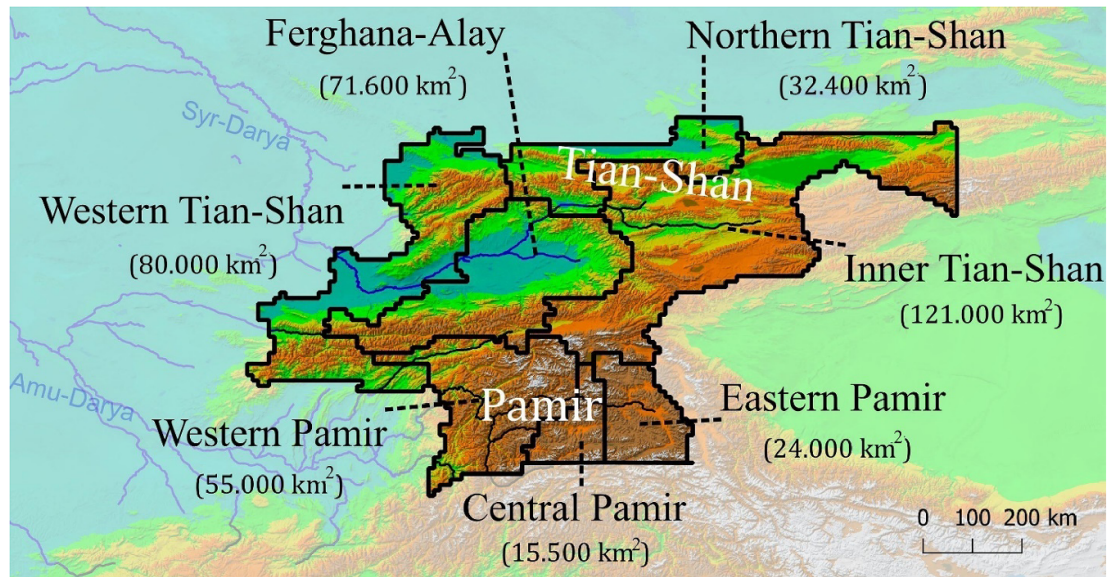
Figure 2. Spatial distribution of the precipitation subregions and their approximate areas. The background colour legend is identical to that in figure 1.
