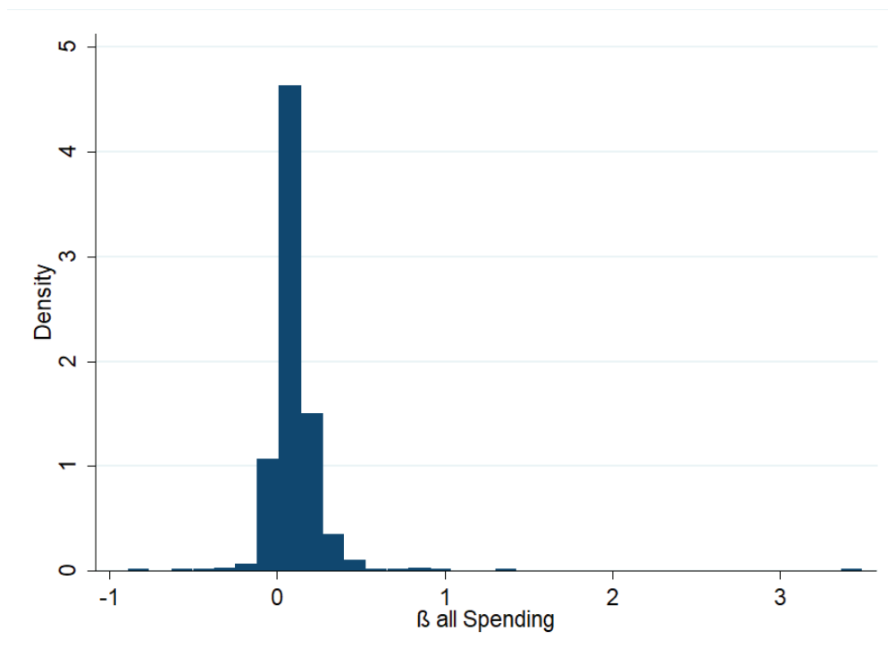
Figure 2: Histogram of \beta for all Spending
