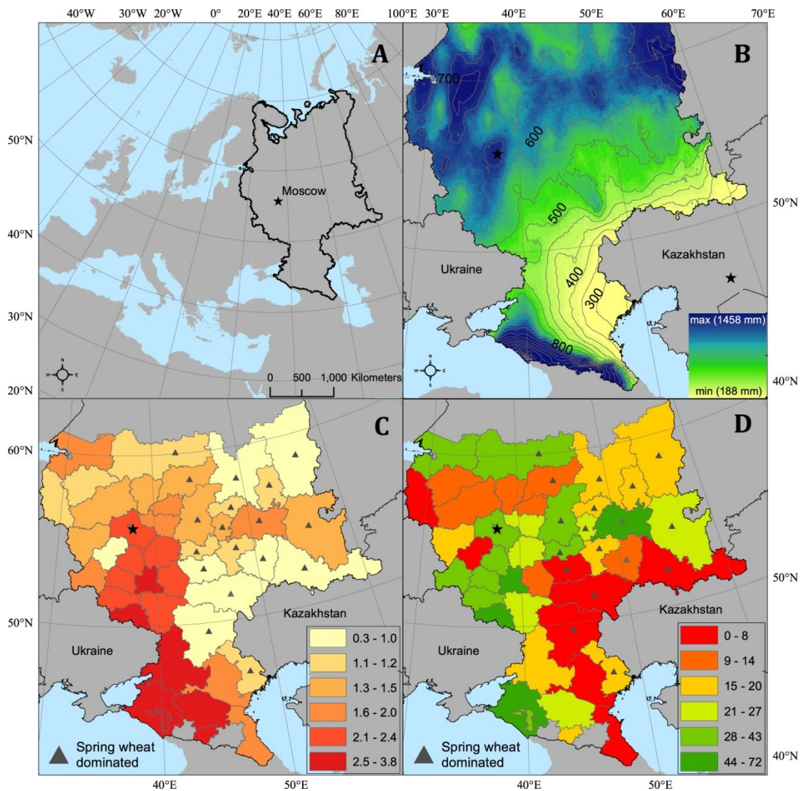
Figure III-1: Study region (A); average annual precipitation (mm) (B); average wheat yields ( t\ ha^{-1} , 1991–2012) (C); average N fertilizer use ( kg/ha , 1991–2012) (D). Data sources: Climatic Research Unit (CRU, TS 1.0 and 2.0, http://www.cru.uea.ac.uk/cru/data/hrg.htm ) (B); ROSSTAT (2014) (C) and (D).
