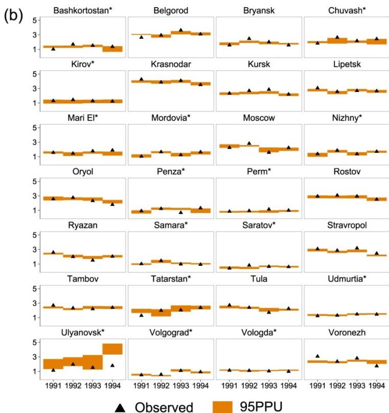
Figure III-4: Comparison of observed yield ( \text{t ha}^{-1} ) with 95PPU of simulated wheat yield ( \text{t ha}^{-1} ) for calibration (A) and validation (B). Asterisk indicates areas dominated by spring wheat.
