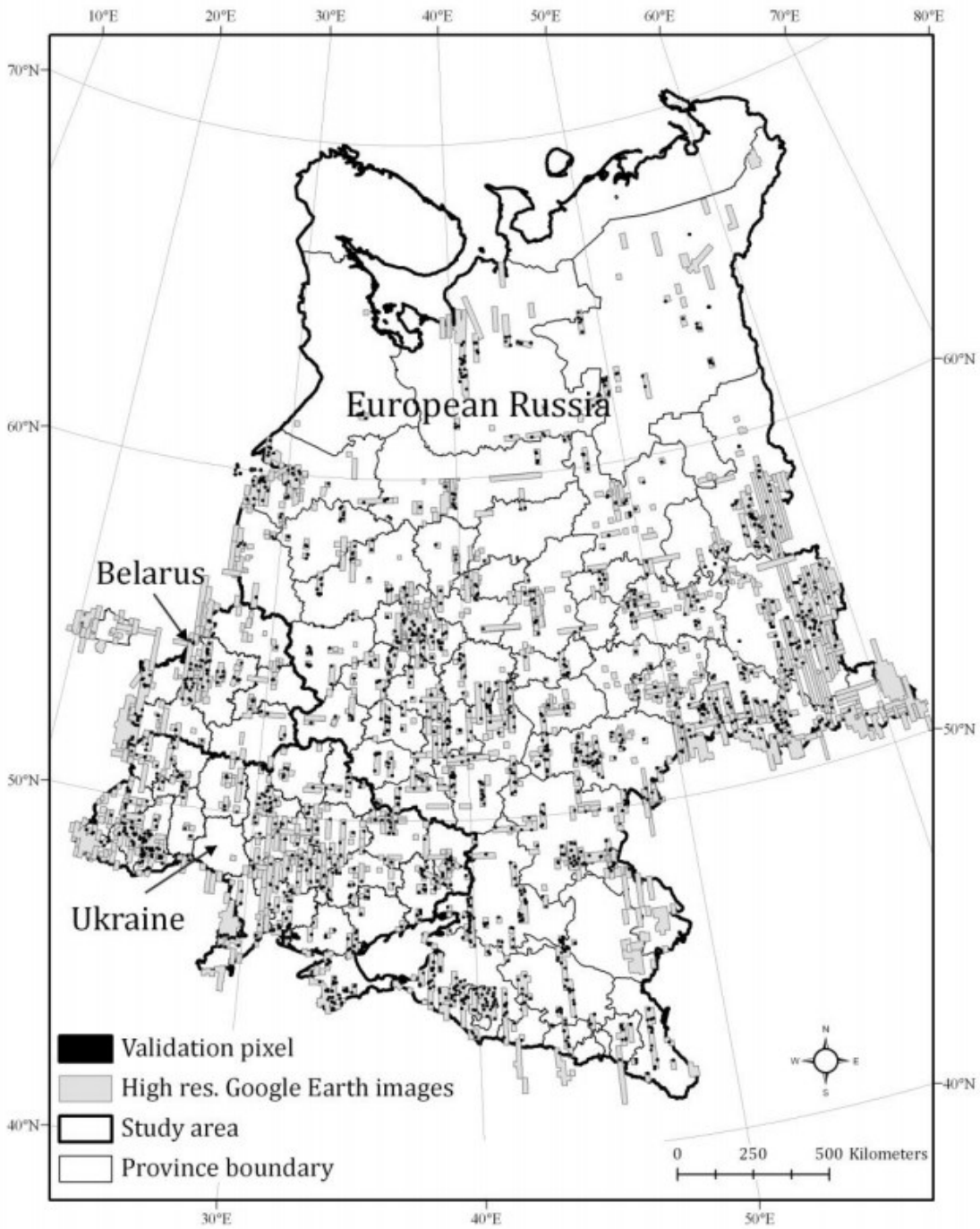
Figure S II-4: Locations of the high-resolution QuickBird and IKONOS images from Google Earth and validation pixels.
