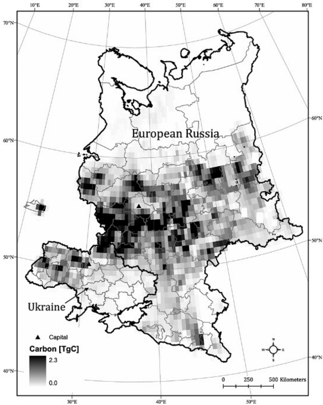
Figure II-7: Spatial distribution of total carbon storage on abandoned cropland between 1990 and 2009. Note that Belarus is excluded because of missing data for cultivated area statistics. Cropland abandonment area and associated carbon sequestration are negligible in Belarus.
