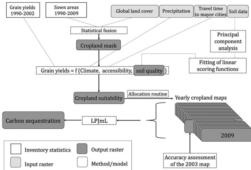
Figure II-1: Method flowchart.
