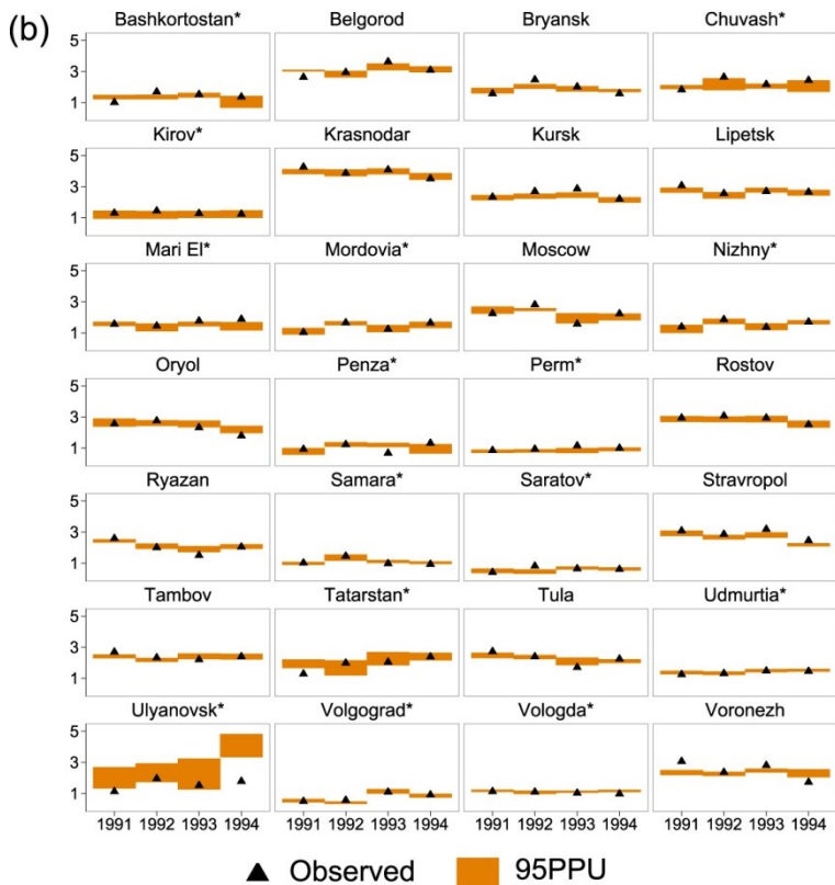
Figure III-4: Comparison of observed yield ( t\ ha^{-1} ) with 95PPU of simulated wheat yield ( t\ ha^{-1} ) for calibration (A) and validation (B). Asterisk indicates areas dominated by spring wheat.
