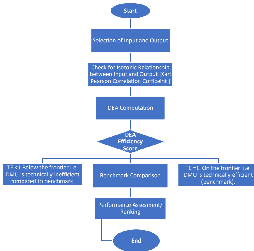
Figure 1: Schema chart of DEA algorithm
